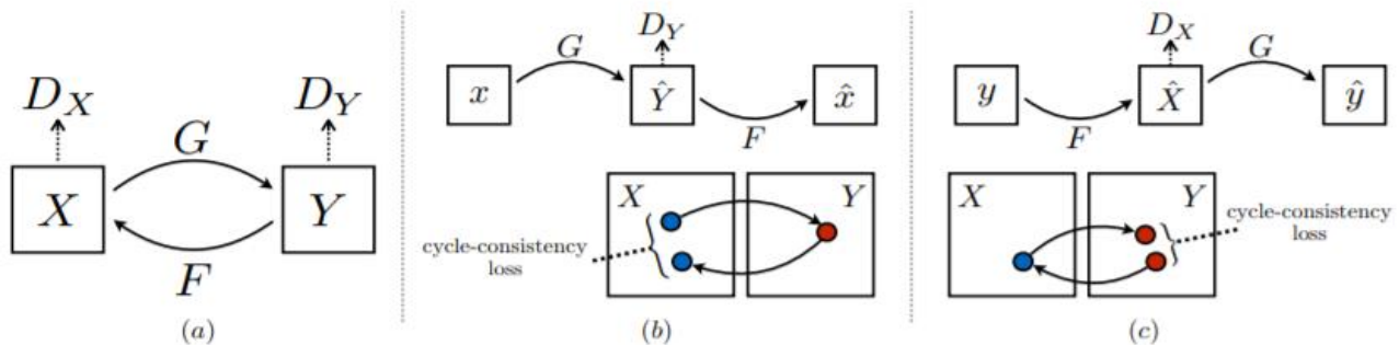
Fig 3: a) Our model contains two mapping functions G : X \rightarrow Y and F : Y \rightarrow X , and associated adversarial discriminators D_Y and D_X . D_Y encourages G to translate X into outputs indistinguishable from domain Y , and vice versa for D_X and F . To further regularize the mappings, we introduce two cycle consistency losses that capture the intuition that if we translate from one domain to the other and back again we should arrive at where we started: (b) forward cycle-consistency loss: x \rightarrow G(x) \rightarrow F(G(x)) \approx x , and (c) backward cycle-consistency loss: y \rightarrow F(y) \rightarrow G(F(y)) \approx y [image source-original research paper[1]]
