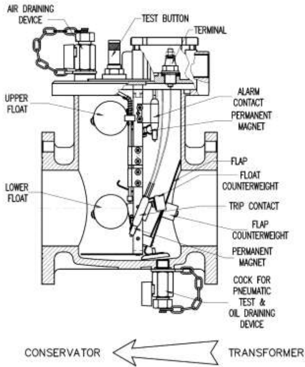
FIG (1) BUCHHOLZ RELAY
