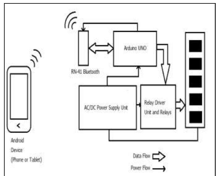
Figure 1. Block Diagram for Android and Arduino Based Switching System
