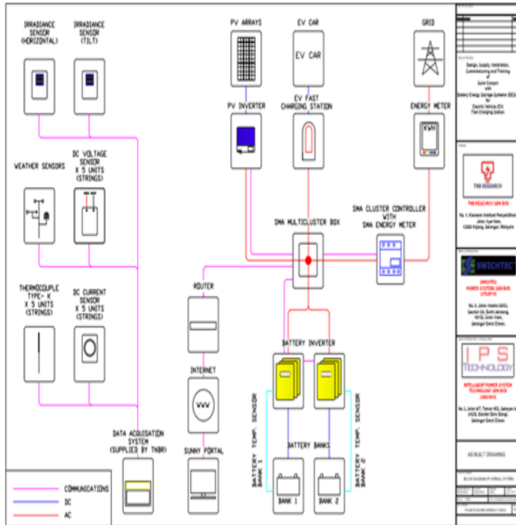
Figure 3: Schematic Block Diagram of the EV
