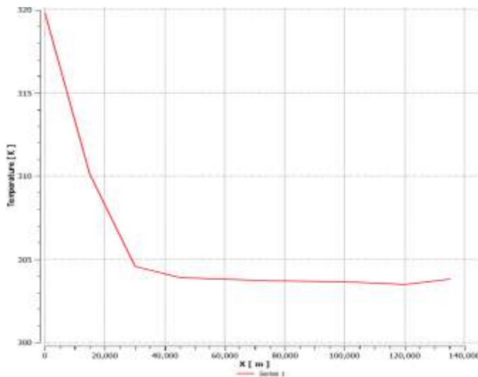
Figure 6: Temperature distribution along the length of the pipeline with Iranian data
