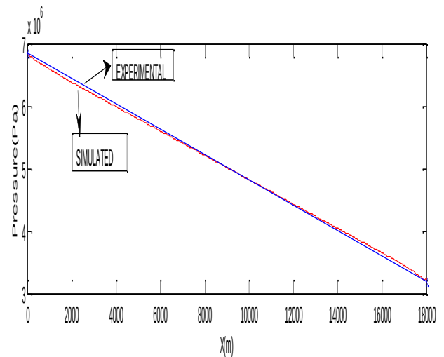
Figure 3: Comparison of simulated pressure distribution along the length of the pipeline with Shell data
