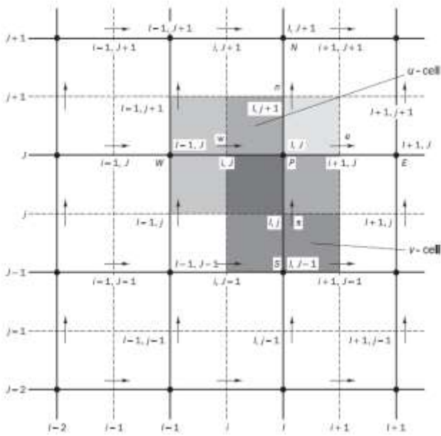
Figure 2: Staggered Structured Grid Arrangement for Pressure and Velocity
