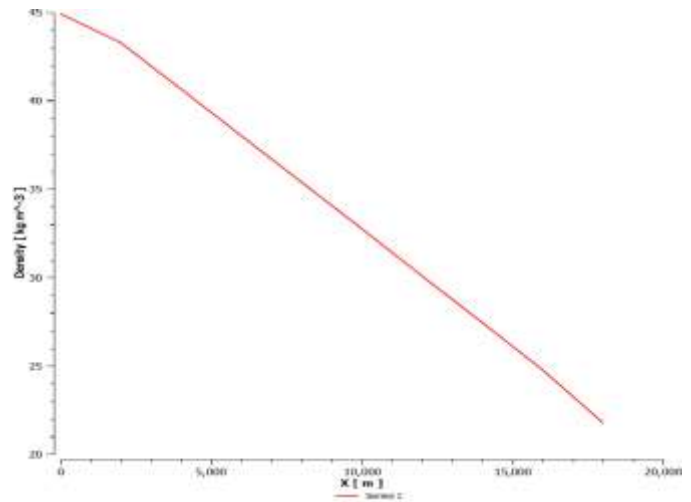
Figure 9: Density distribution along the length of the pipeline with Shell data
