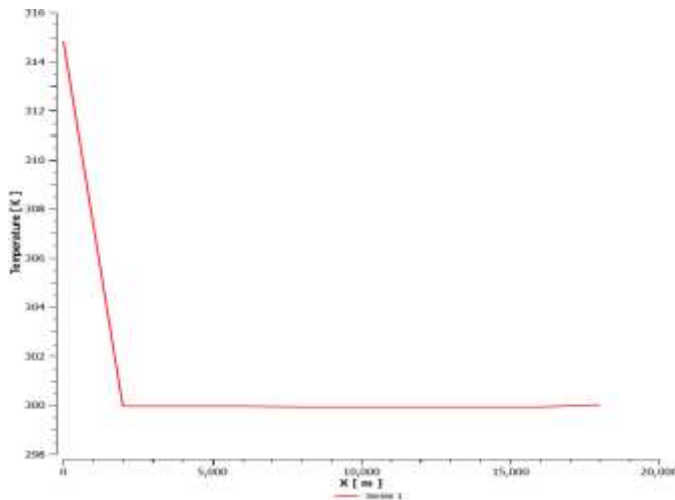
Figure 5 Temperature distribution along the length of the pipeline with Shell data
