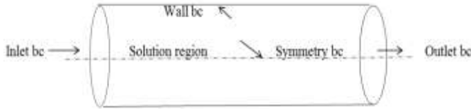
Figure 1: Flow domain and boundary conditions (Noorbehesht, 2012)
