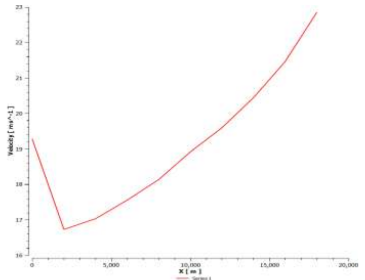
Figure 7: Velocity distribution along the length of the pipeline with Shell data
