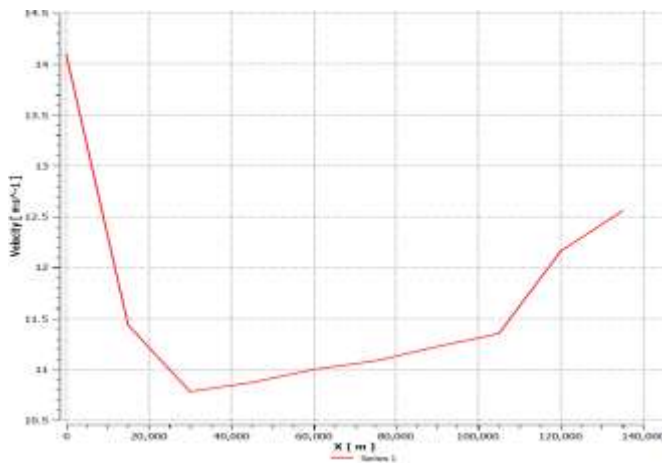
Figure 8: Velocity distribution along the length of the pipeline with Iranian data.
