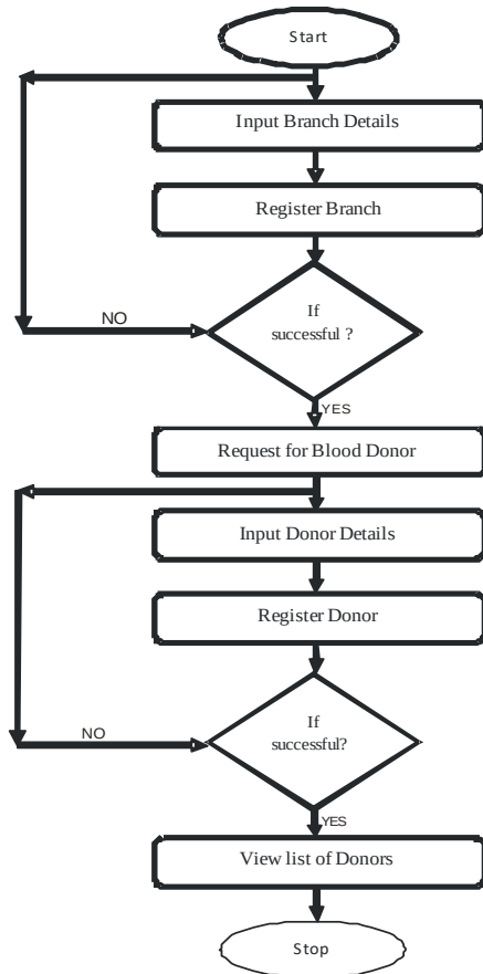
Figure 2. System's Flowchart
