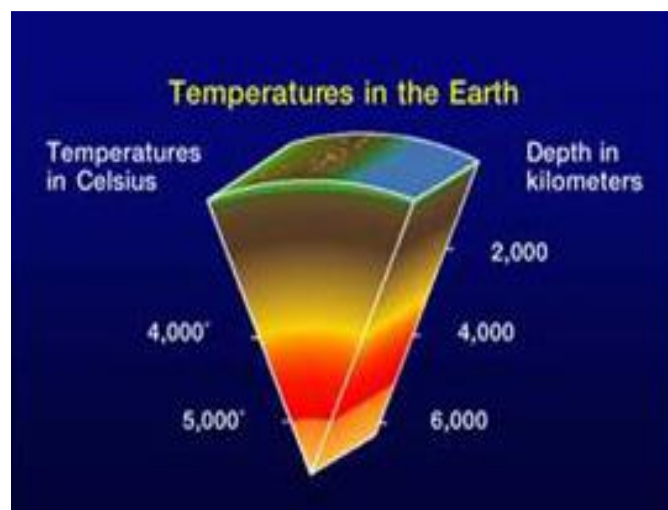
Figure1. Temperatures in the earth (from Energy and Geosc. Inst. 1997).
