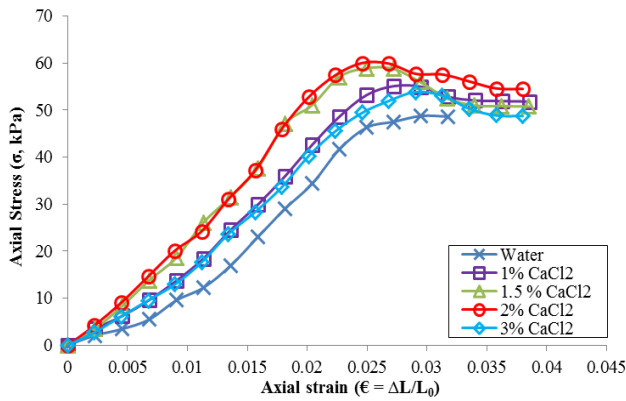
g) Soil C (100%BCS) at w_i = 28.60\%
