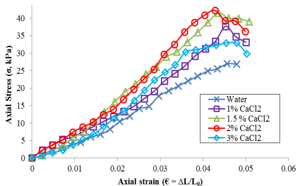
i) Soil C (100%BCS) at w_i = 14.64\%
