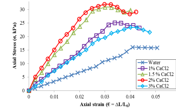
f) Soil B (80%BCS+20%Bentonite) w_i = 19.52\%
