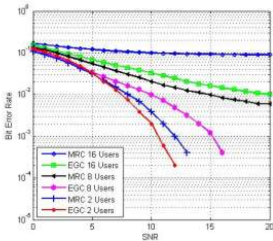
Fig 6. BER Vs SNR performance comparison of MC-CDMA with EGC and MRC using BPSK over Rayleigh channel
