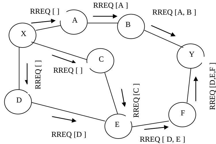
Fig. 1. RREQ message flow in EE-HRP
