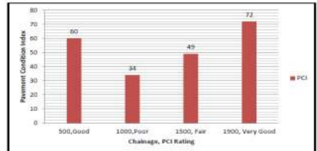
Figure 9: PCI for every 500m length of stretch-1
