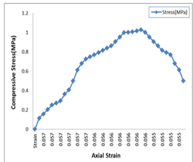
Fig.5.9: Compressive Stress and Axial Strain Curves For 21 Days Curing Period with FA=80%, C/FA=20% and C/OPA=8% Mix Ratios
