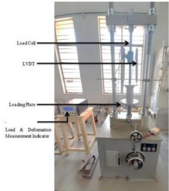
Fig.4.3: Experimental Setup of Compression Testing Machine
