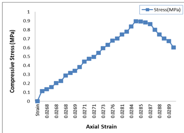
Fig.5.14: Compressive Stress and Axial Strain Curves For 14 Days Curing Period with FA=50%, C/FA=40% and C/OPA=20% Mix Ratios
