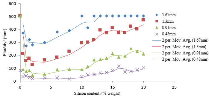
Figure 2: Fluidity as a function of silicon content and test channel modulus
