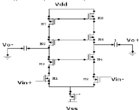
Figure 4.1: Telescopic Amplifier
