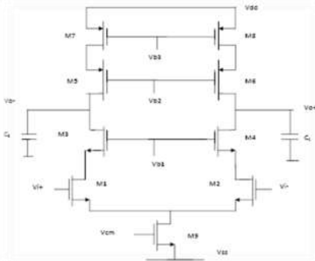
Figure 1.1: Telescopic differential amplifier
