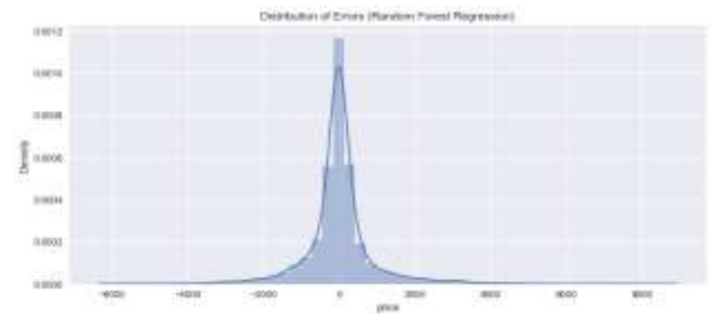
Fig. 16. Distribution of Errors Random Forest Regression
