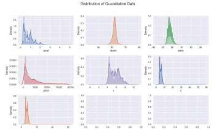
Fig. 2. Distribution of Quantitative
