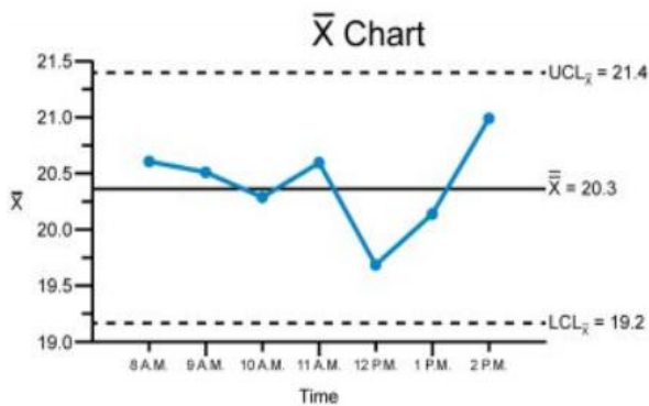
Control Chart
