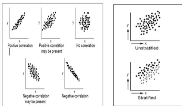
Scatter Diagram
