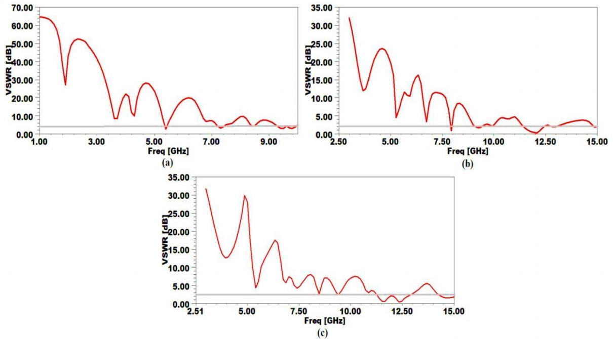
Fig.8. VSWR vs. Frequency plot at feed position (a) (-10, 0), (b) (4, -8) and (c) (2, -10)
