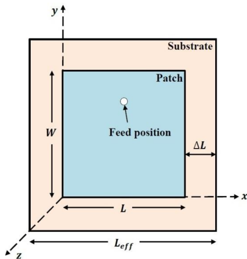
Fig.2. 2D view of probe fed microstrip patch antenna
