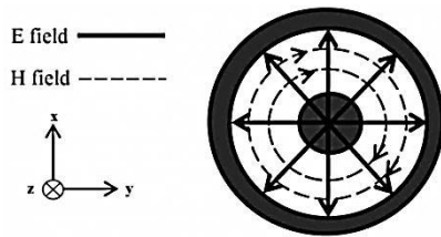
Fig.1. E and H fields on the coaxial line
