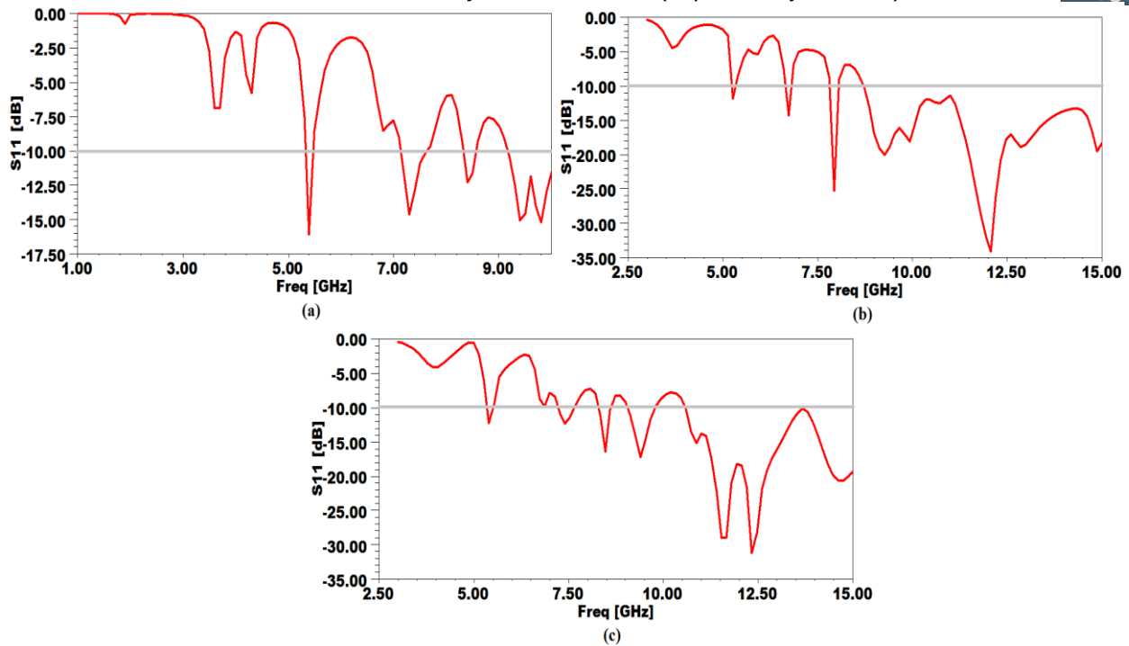
Fig.6. Return loss vs. frequency plot of proposed antenna with feed position (a) (-10, 0), (b) (4, -8) and (c) (2, -10)
