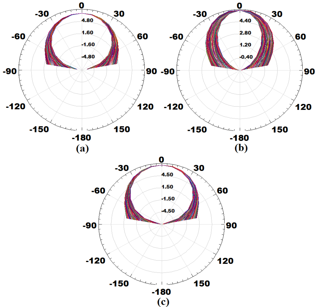
Fig.7. Far field radiation pattern of proposed antenna with feed position (a) (-10, 0), (b) (4, -8) and (c) (2, -10)
