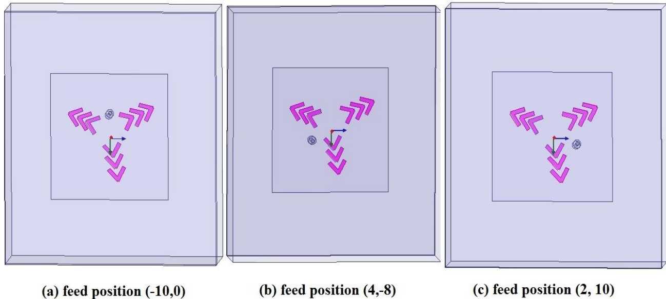
Fig.5. Top view of proposed antenna with varied feed positions
