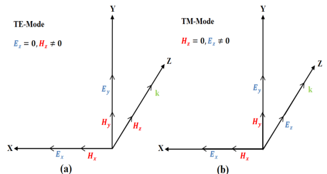
Fig.3. Components of EM fields in a rectangular waveguide: (a) TE mode E_z = 0 , (b) TM mode H_z = 0
