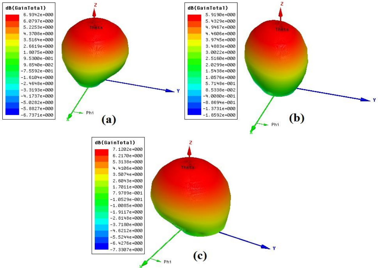
Fig.9. 3-D polar plot of gain of proposed antenna at feed position (a) (-10, 0), (b) (4, -8) and (c) (2, -10)
