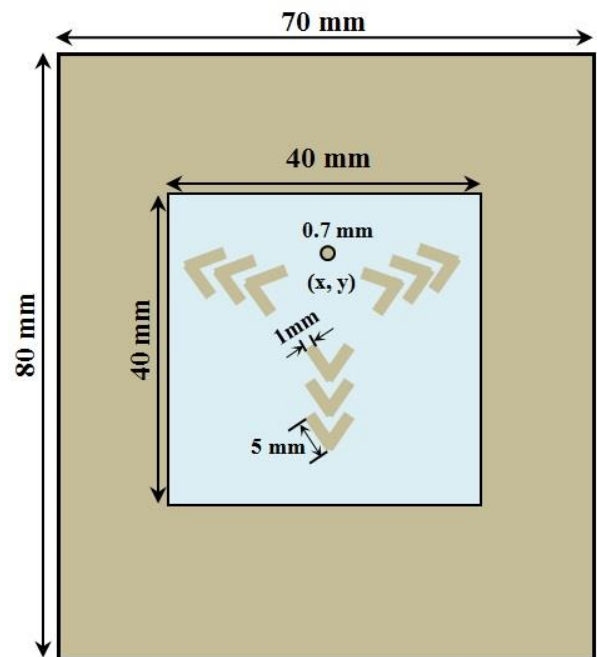
Fig.4. Dimensional view of designed antenna
