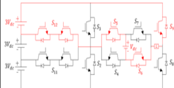
Fig. 3.1(xvi) Equivalent Circuit of Mode 16
