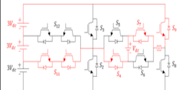
Fig. 3.1(xvii) Equivalent Circuit of Mode 17
