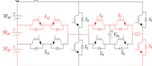
Fig. 3.1(vii) Equivalent Circuit of Mode 7
