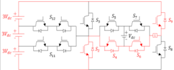
Fig. 3.1(xxi) Equivalent Circuit of Mode 21
