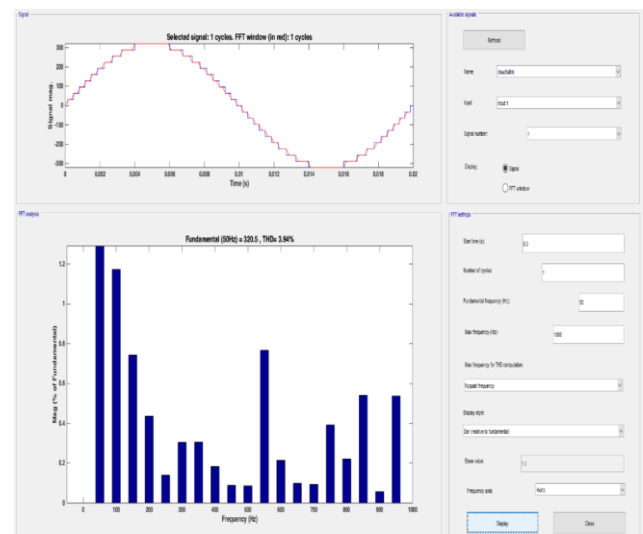
Fig. 7. (i) Output voltage waveform for resistive load R=22\ \Omega and full load current I_L=10\ A (ii) THD analysis of output voltage waveform using half height method
