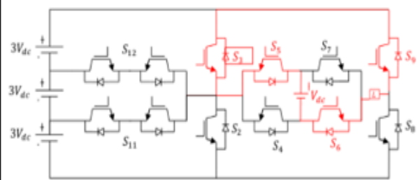
Fig. 3.1(xiii) Equivalent Circuit of Mode 13
