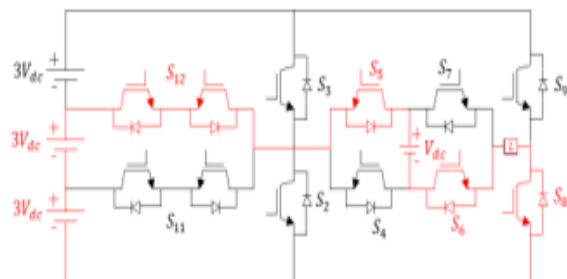
Fig. 3.1(vi) Equivalent Circuit of Mode 6
