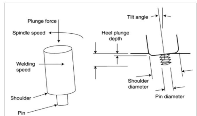
Fig.8 Tool geometry.
