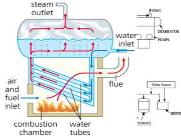
Fig. 2. A Simple water tube boiler[15]
