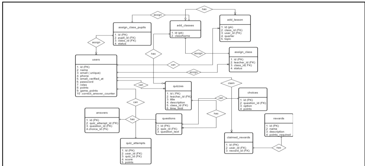
Figure 10. Entity-Relationship Diagram
