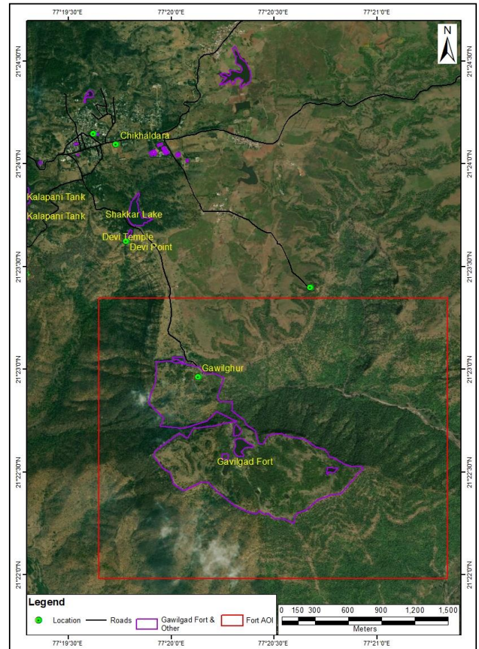
Fig. 7. Transport map of Gawilghat Fort
