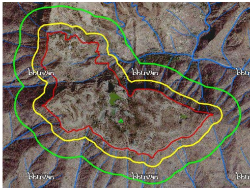
Fig. 9. Drainage & with three buffers & Gawilgarh Fort
