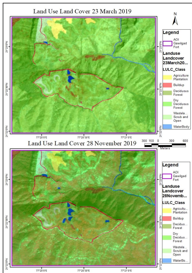
Fig. 6. Land use Land Cover Map of Gawilghat Fort
