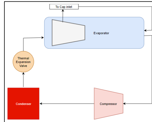
Fig 2. Layout of proposed setup
