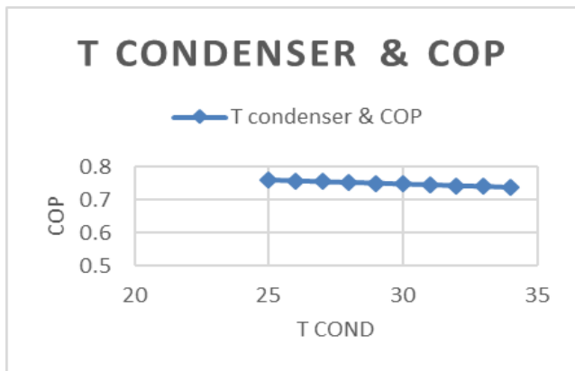
Fig. 18 Effect of Condenser Temperature T_{15} on COP at \varepsilon_{sh,x} = 0.64 and \dot{m}_1 = 1.5 \text{ kg/s}
