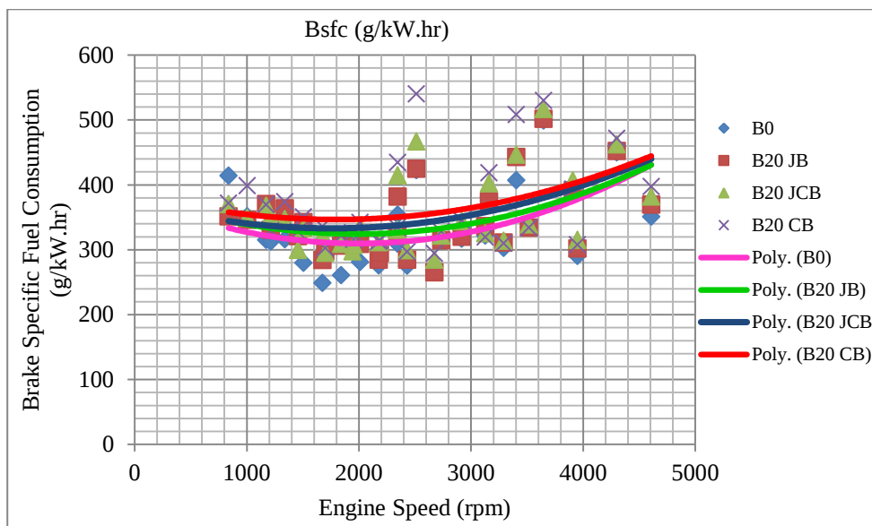
Fig.5. Comparison of Bsfc vs. engine speed for tested fuel samples
