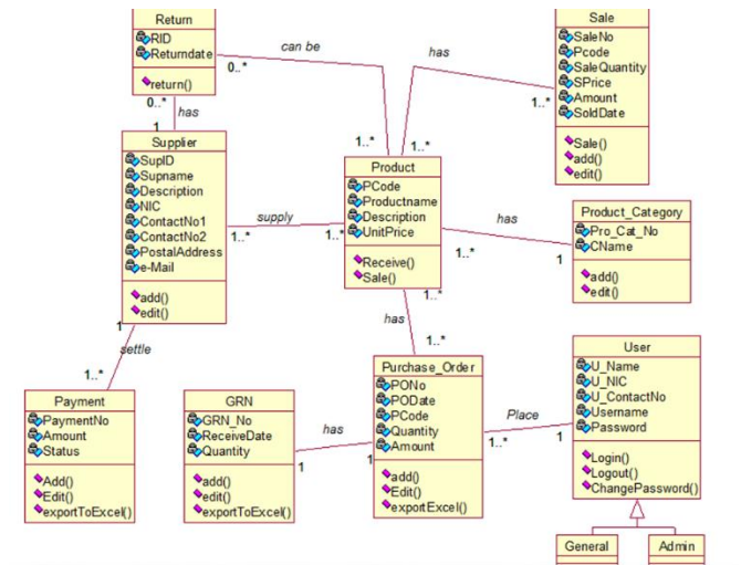
Figure 2. Class diagram
