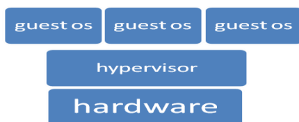
Fig.1. Virtual Machine
