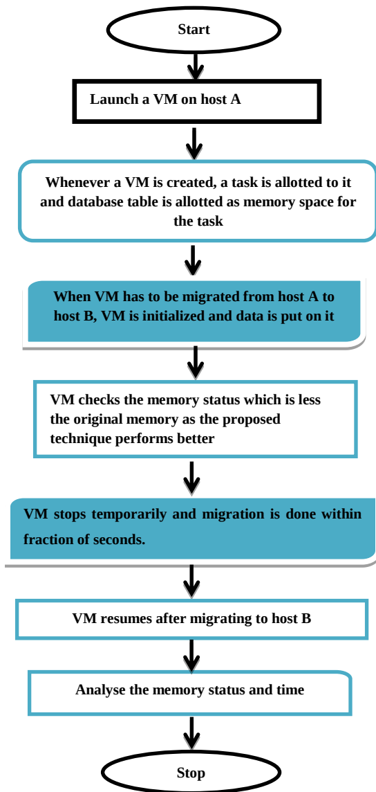
Fig.4. Proposed Methodology
