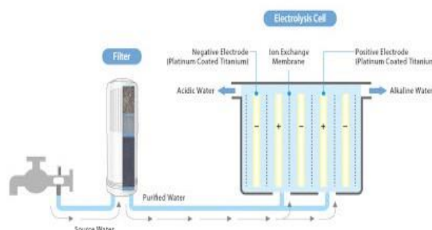
Fig.1 Electrolysis or ionization proses of ionizer
