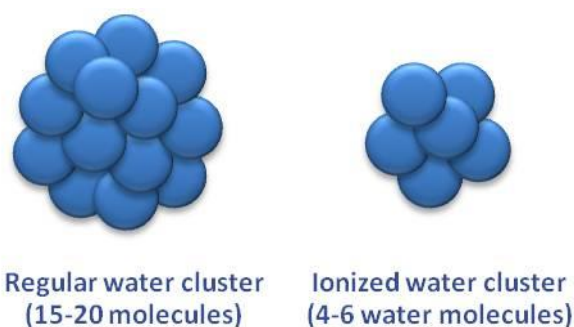
Fig.5 Water Cluster Molecules in normal water and in Hydrokalkine water
