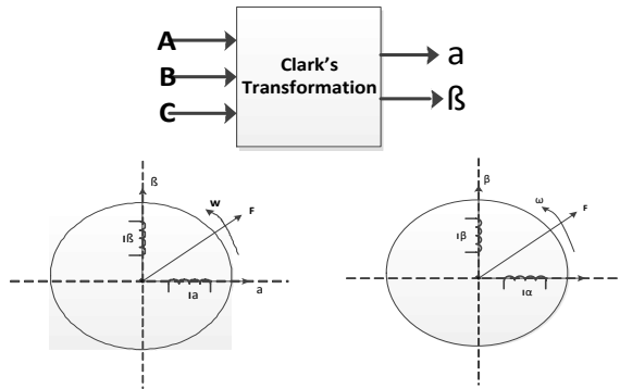
Fig 1 Clark's Transformation
