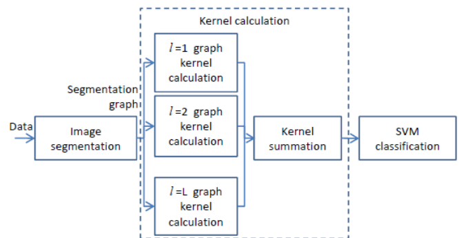
Fig. 5. SVM 'Kernel' Classification [14]
