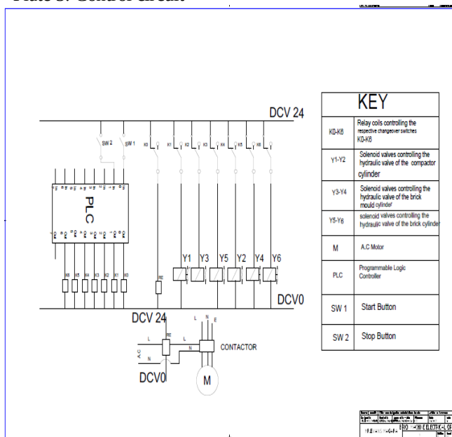
Plate 3: Control circuit
