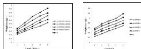
Fig. 6a) Effect of applied load on weight loss with WC and Graphite b) Effect of applied load on weight loss with WC only
