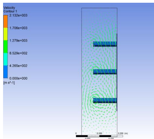
Fig. 8. Contour Velocity for stator blades without cuts
