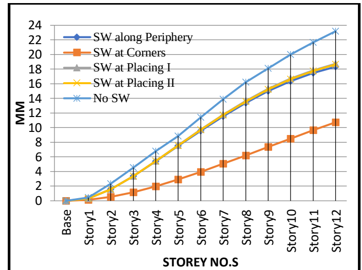
Fig.11. Storey Displacement
