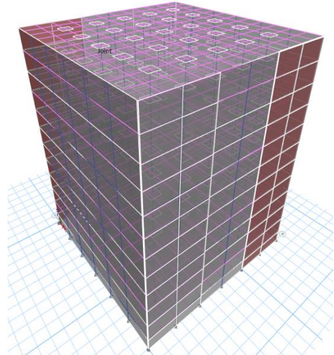
Fig.6. 3D View of SW Placing II
