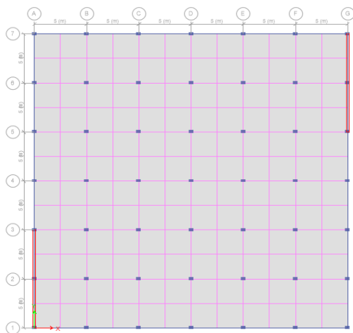
Fig.5. SW Placing II
