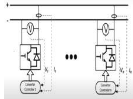
Fig.2 Autonomous control
