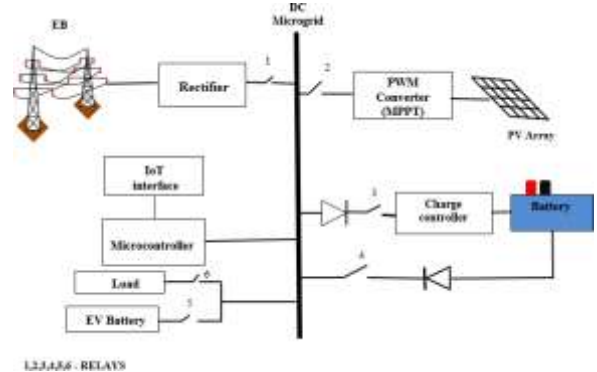
Fig.4 Proposed System Configuration
