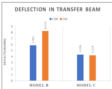
Fig. 15. Deflection in transfer beams
