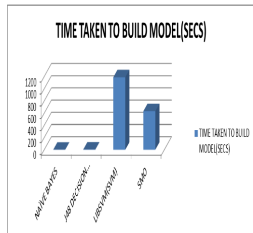
Fig. 5. A Graph of Different types of Algorithm as against time taken to build the model (secs) for 19 attributes
