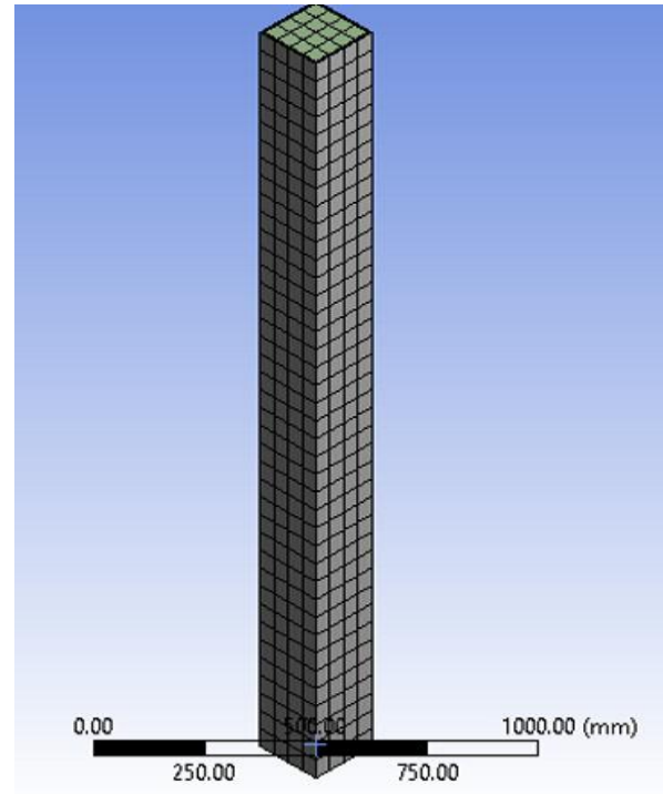
Fig.2. Meshing of square CFST column
