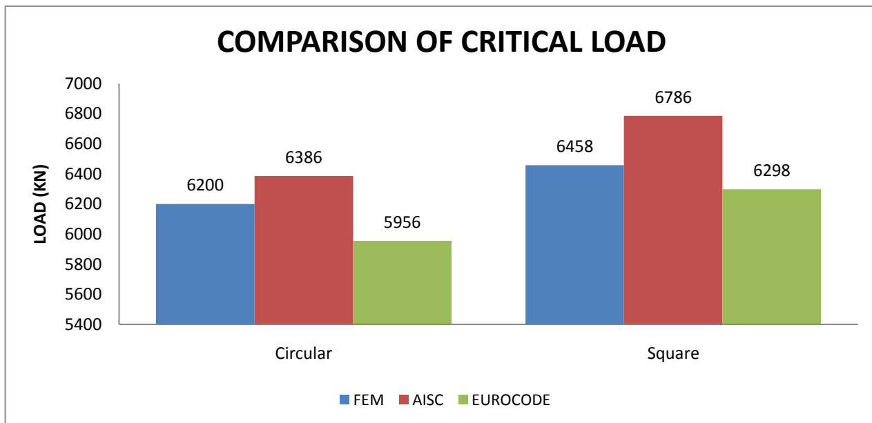
Chart 5. Critical load comparisons of slender CFST columns (L=4000mm)
