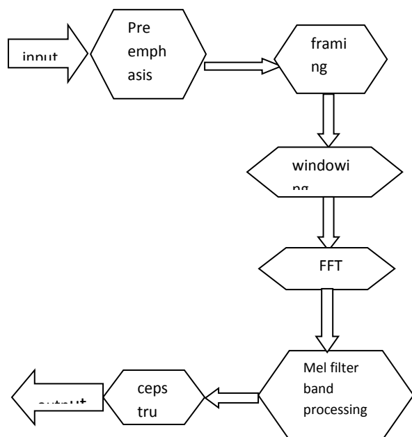
Figure 1: Block diagram of MFCC
