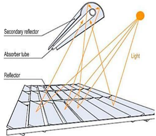
Figure 1.5 Linear Fresnel reflector e
