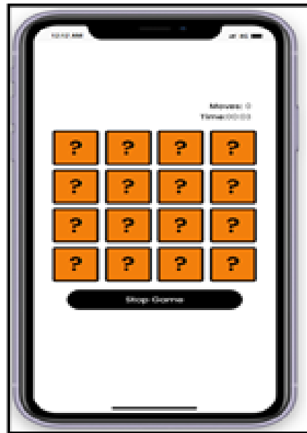
Figure 16. Memory Game
