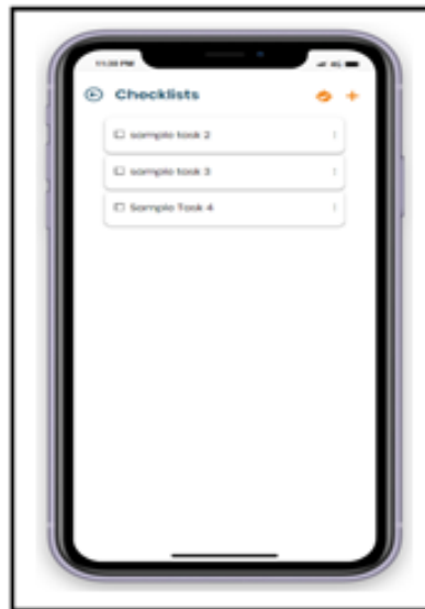
Figure 9. Checklist Dashboard
