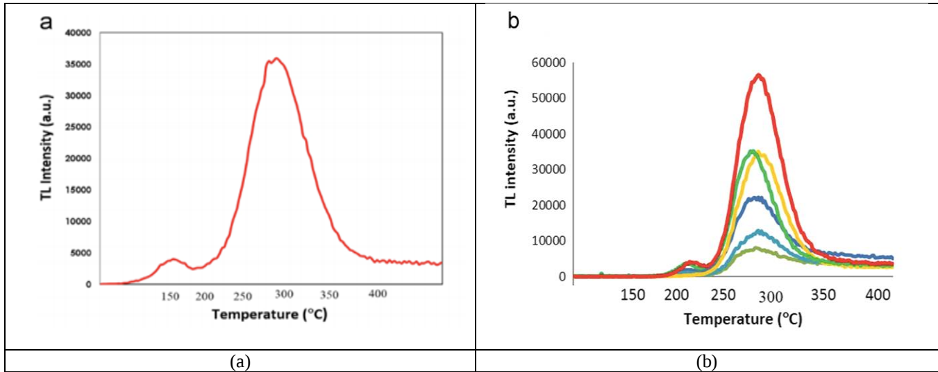
Figure 1. Thermoluminescent (TL) glow curves of BeO irradiated with ^{90}\text{Sr}/^{90}\text{Y} beta radiation. (a) 100 mGy; (b) Different doses.
