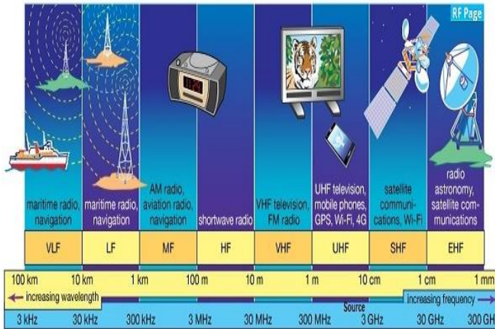
Figure 1. Frequency applications
