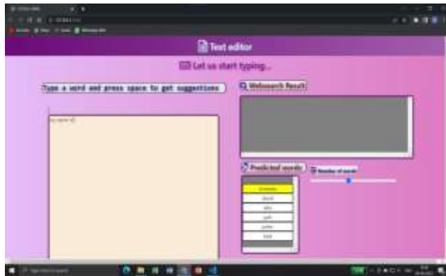
Fig 4 LSTM Prediction
