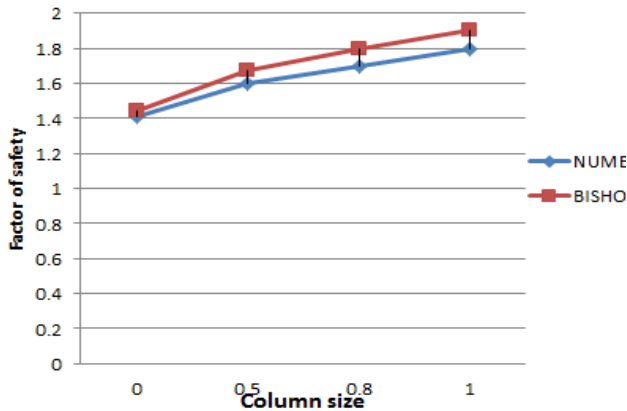
Figure 8.The influence of the size of DM columns
