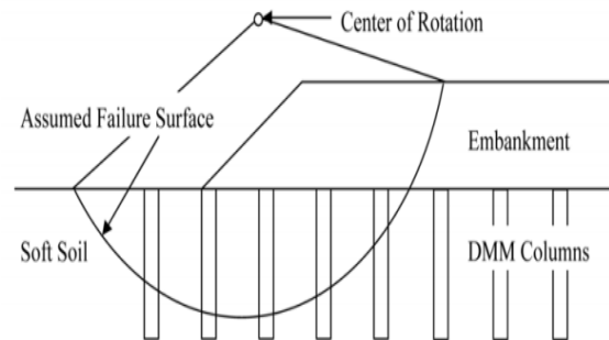
Figure 1 Circular sliding surface (after Broms and Boman 1979)
