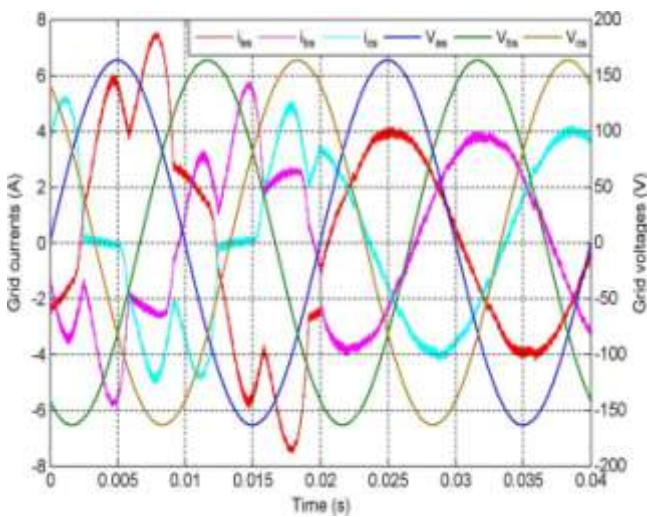
Fig.6. Grid currents after compensation with the algorithm from [14]
