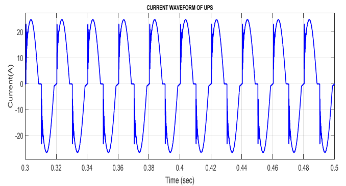
Fig. 11. (b) Supply current waveform of UPS
