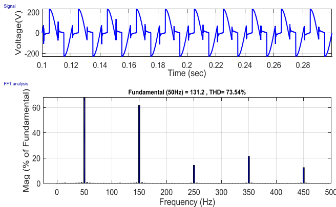
Fig. 10. (c) Voltage THD ( THD_v ) of fan
