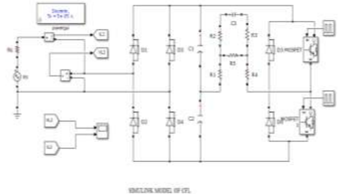
Fig. 2. Simulation model of CFL
