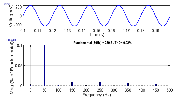
Fig. 11. (c) Voltage THD ( THD_v ) of UPS
