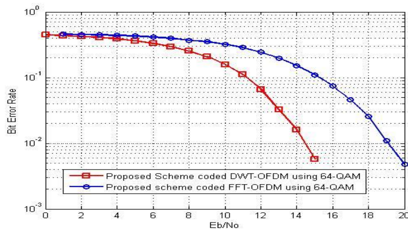
Figure 4 Performance of proposed scheme coded DWT-OFDM system as compare to Proposed scheme coded FFT-OFDM using 64-QAM modulation
