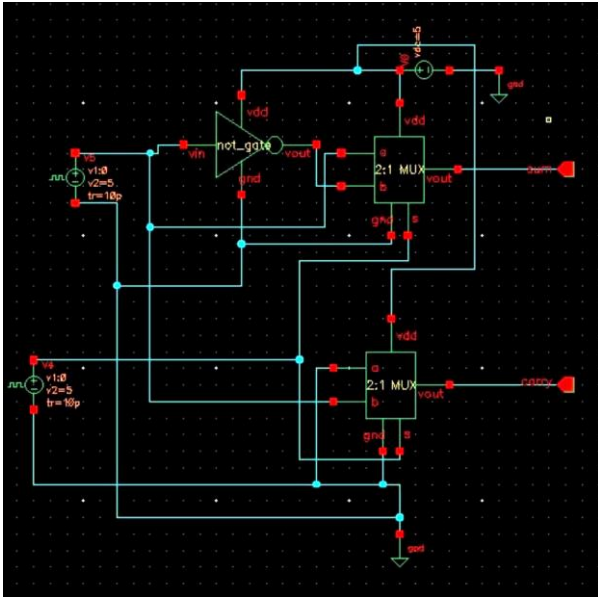
Fig.5 A half adder implemented using NMOS pass transistors logic on cadence virtuoso [1].
