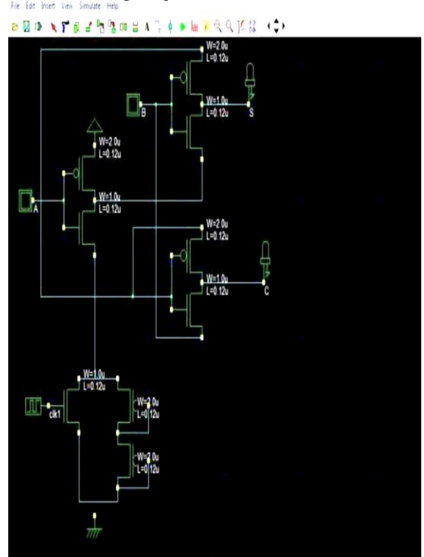
Fig.6 Half Adder Circuit diagram using the AVLG Techniques [2].
