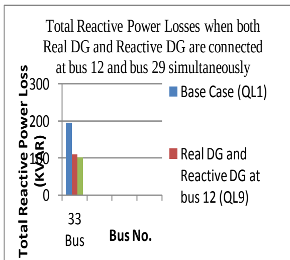
Fig. 17 Reactive power loss comparison when both real and reactive DGs are connected at same
