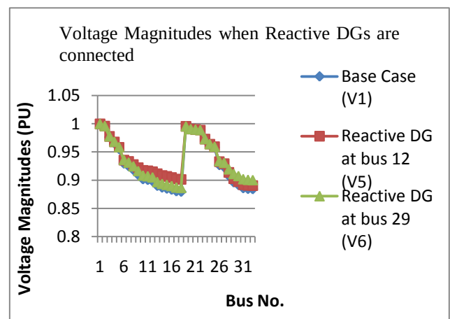
Fig. 6. Voltage comparison when reactive DG is connected
