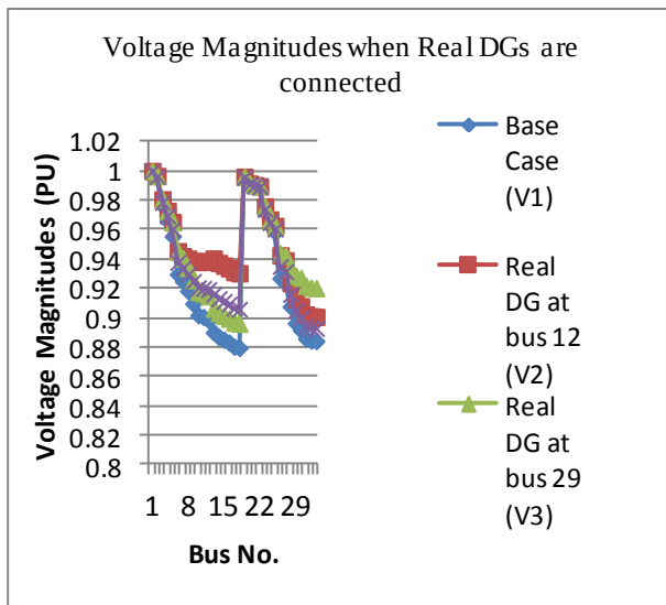
Fig. 3. Voltage comparison when real DG is connected
