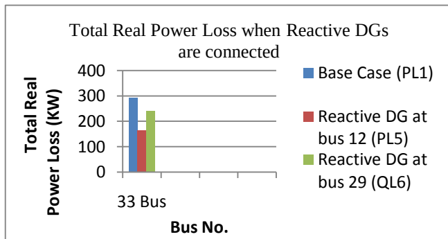
Fig. 7 Real power loss comparison when reactive DG is connected
