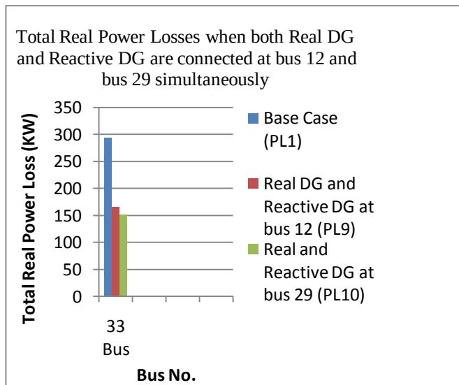
Fig. 16 Real power loss comparison when both real and reactive DGs are connected at same bus
