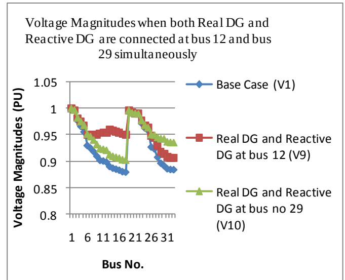
Fig. 14 Voltage comparison when both real and reactive DGs are connected at same bus
