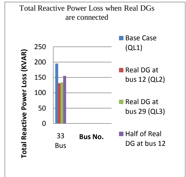
Fig.5. Reactive power loss comparison when real DG is connected
