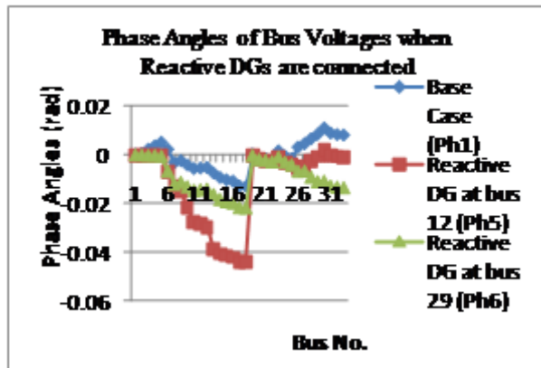
Fig.9. Phase angle comparison when reactive DG is connected
