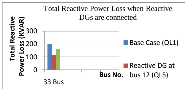
Fig. 8 Reactive power loss comparison when reactive DG is connected
