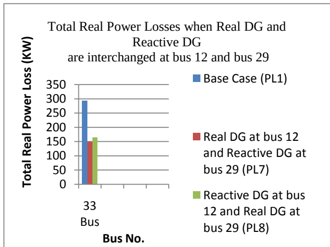
Fig. 12 Real power loss comparison when real DG and reactive DG are interchanged
