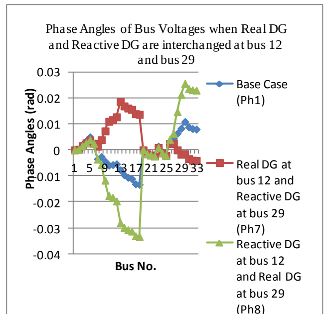
Fig. 11 Phase angle comparison when real DG and ractive DG are interchange
