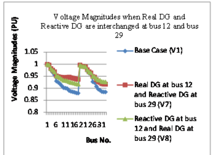
Fig. 10 Voltage comparison when real DG and reactive DG are interchange
