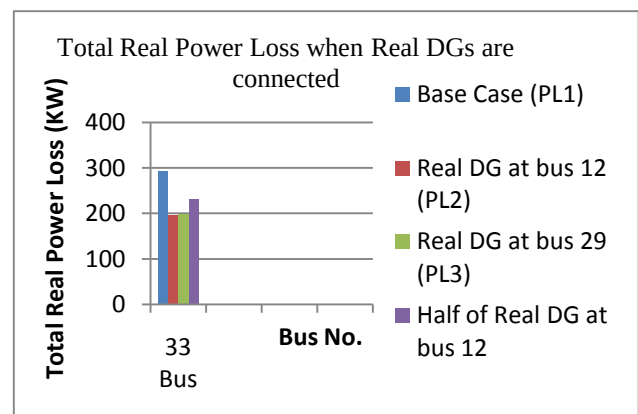
Fig.2.Real power loss comparison when real DG is connected
