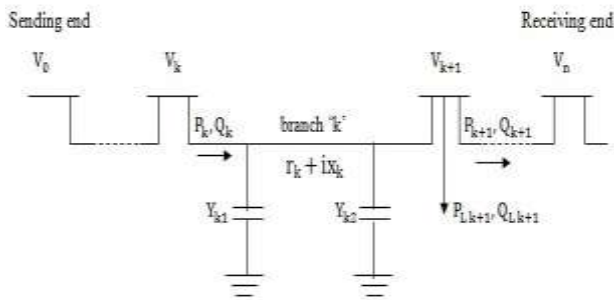
Fig. 1. Single line diagram the radial distribution system
