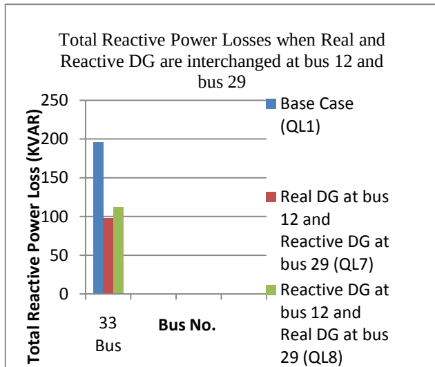
Fig. 13 Reactive power comparison real DG and reactive DG are interchanged
