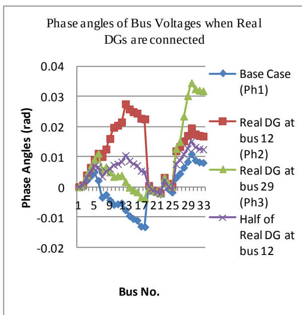
Fig. 4. Phase angle comparison when real DG is connected
