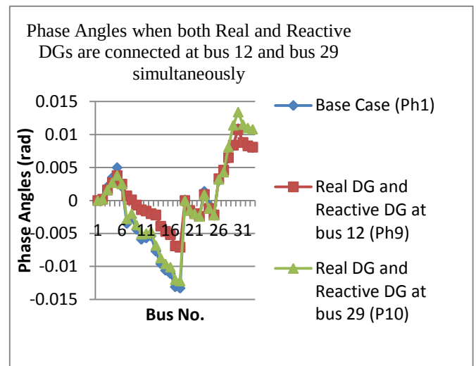
Fig. 15 Phase angle comparison when both real and reactive DGs are connected at same bus
